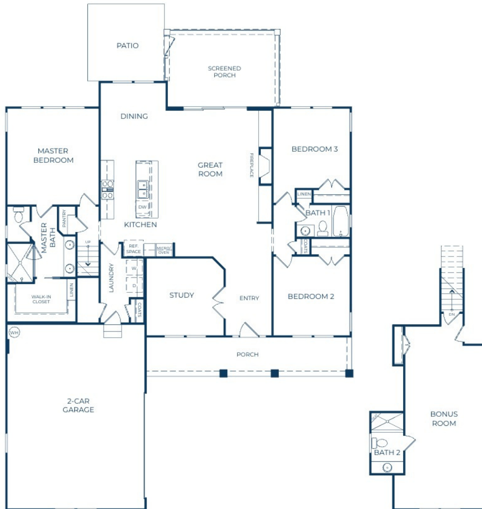
ELEVATION COASTAL FIRST FLOOR
